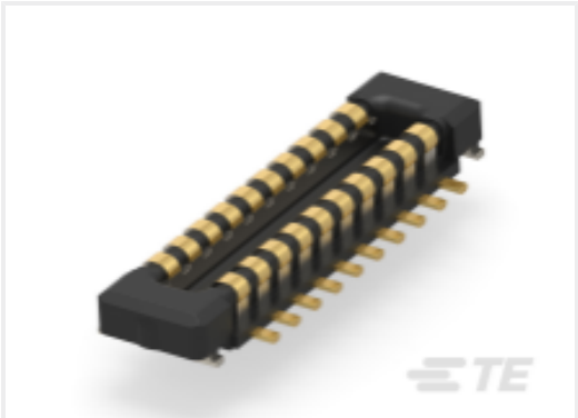
TE 产品编号2-2363962-0 0.4mm BTB CONN H0.8 PLUG ASSEMBLY, 20P
