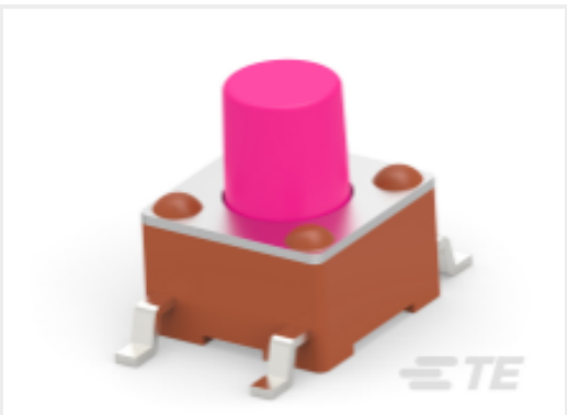
TE 产品编号2-1977223-0 FSM6JSMASTR=6MM TACT SWITCH, SMT 260gf
