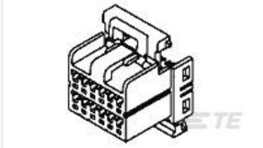
TE 产品编号174045-2 040 MULTILOCK PLUG 12P
