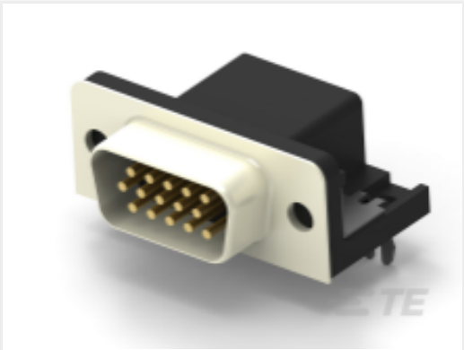
TE 产品编号2311774-1 AMPL PLUG, HD22, R/A, 15P, THREADED
