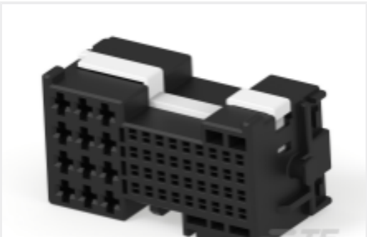
TE 产品编号2109452-2 050/110 48P PLUG ASSY CODE A
