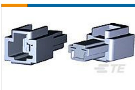
TE 产品编号1-172127-1 FF 250 REC HSG 1P NYLON NAT
