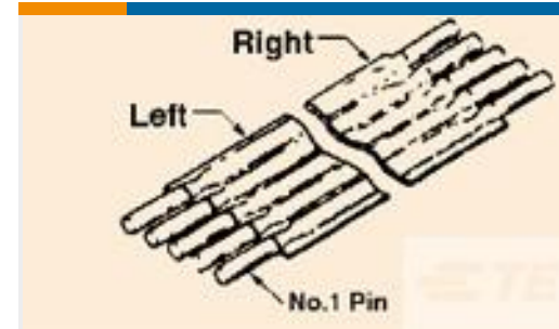
TE 产品编号7-1447183-8 FSN-2.5A-13=JUMPER NOMEX
