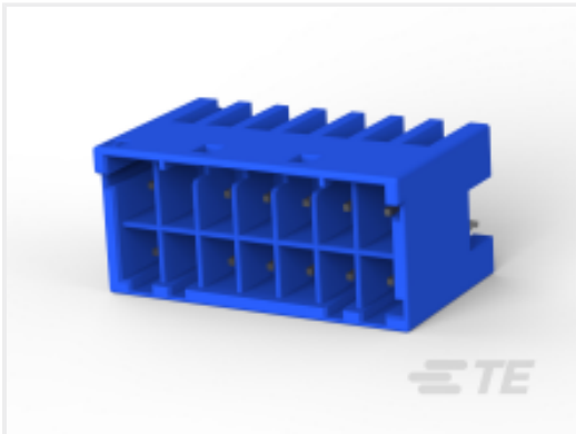
TE 产品编号 6-1971906-7 HEADER ASSY 14POS,KEYING-B,NEW GIC3.3
