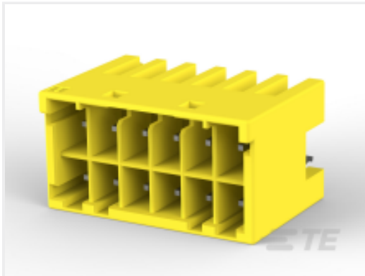
TE 产品编号 4-1971906-6 HEADER ASSY 12POS,KEYING-D, NEW GIC3.3
