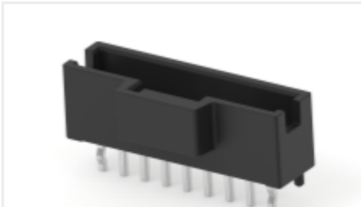
TE 产品编号5-1971817-7 7P,RAST 2.5 Tab Header,Ex- Locking, THV
