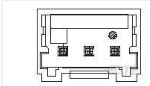
TE 产品编号1-1971032-3 3POS HEADER ASSEMBLY FOR GIC 2.0 EV
