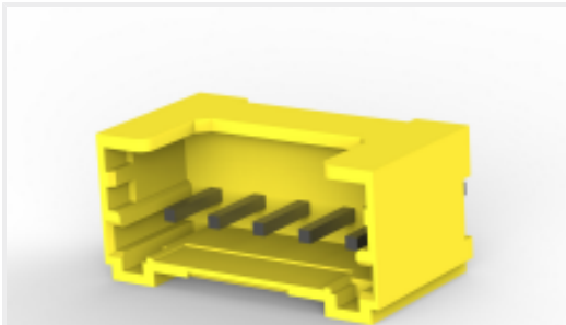
TE 产品编号3-1971032-5 5POS HEADER ASSEMBLY FOR GIC 2.0 EV
