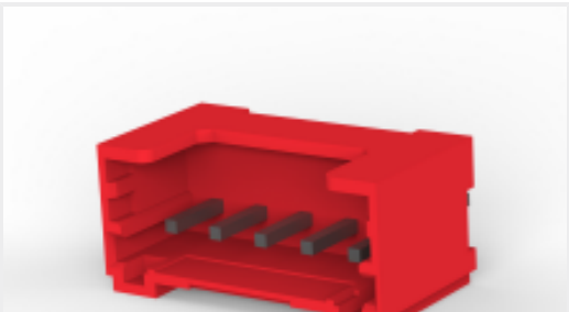
TE 产品编号1-1971032-5 5POS HEADER ASSEMBLY FOR GIC 2.0 EV
