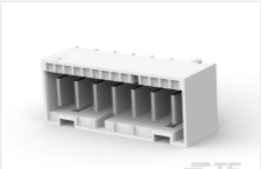
TE 产品编号2232532-7 7P, PL RAST 5 Tab Header, TH,Vertical
