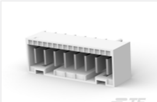
TE 产品编号2232532-8 8P, PL RAST 5 Tab Header, TH,Vertical
