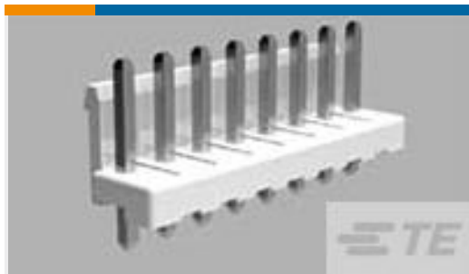
TE 产品编号640454-3 PCB Header: Polyester, Vertical, 2.54 mm
