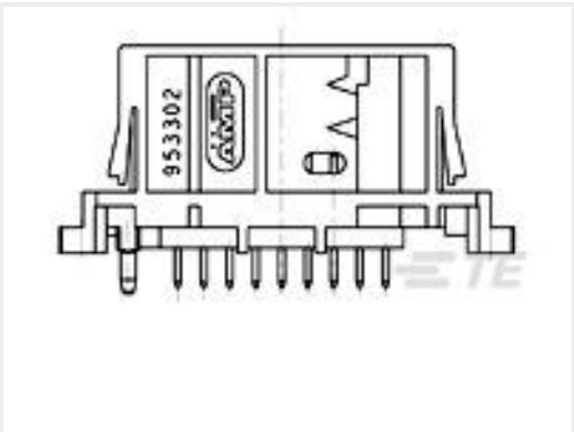
TE 产品编号953302-1 18pos MQS .63 header 180deg
