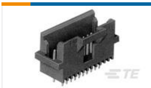
TE 产品编号104666-6 100 SYSTEM 50 HDR DRST SHRD
