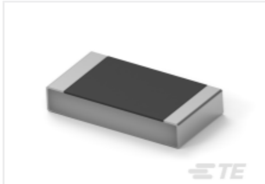
TE 产品编号6-2176458-5 CPF 1206 4R64 0.1% 25ppm 1K RL
