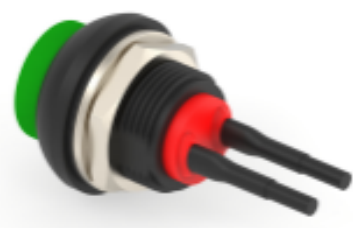
TE 产品编号2329359-9 PB ON/OFF HC GRE M1 TERM IP68 500MM LHS
