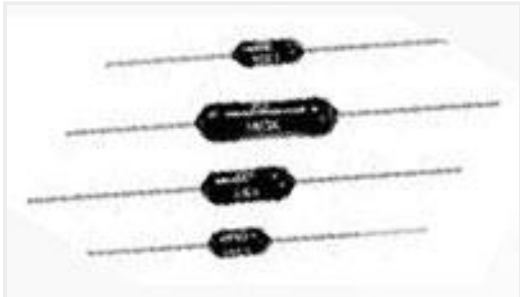
TE 产品编号3-1879627-8 H4P 360R 1% 100PPM
