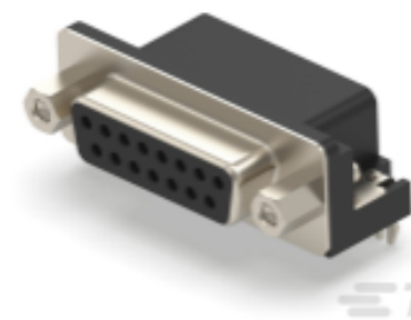
TE 产品编号2301845-2 AMPL REC HD20, R/A, 15P, B/L, 4-40 A /LOCK
