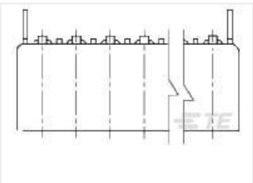
TE 产品编号5-487508-7 TRIOMATE ASY H 8P L=3.175,LDFR
