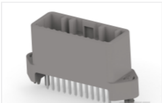
TE 产品编号1802828-2 24W TH HEADER ASSY GREY
