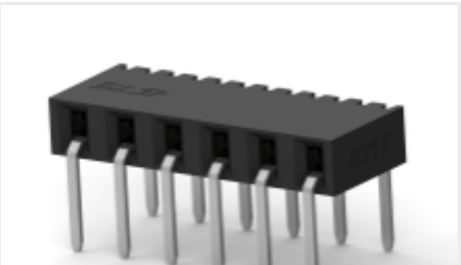
TE 产品编号2314936-6 6P,2MM,B-B,REC,SRHZ,2.8,0.1AU,TR
