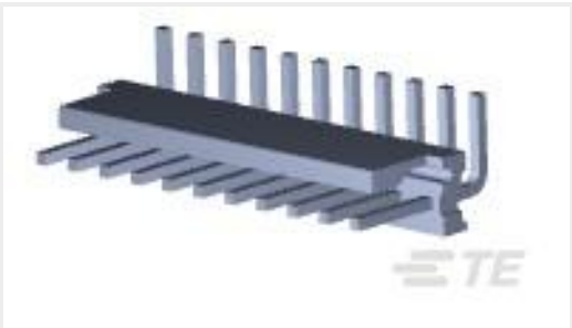
TE 产品编号1-640387-1 11P MTA156 HDR ASSY SQ R/A
