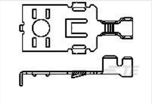
TE 产品编号63496-1 POWER RING TERMINAL TAB 16-10 AWG BR
