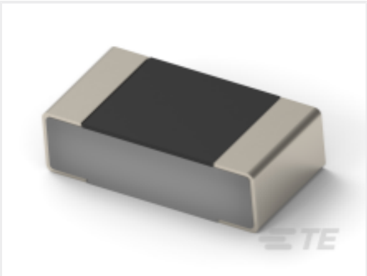
TE 产品编号1-2176467-9 TLRP 1206 1.0W R030 1% 75PPM 5K RL
