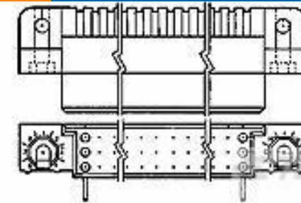
TE 产品编号5533268-3 ASSY,RECPT,R.ANGLE,HDI,LEAD-FR
