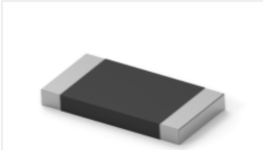
TE 产品编号1-1614958-4 CPF 0805 1R33 0.1% 25ppm 1K RL
