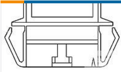
TE 产品编号103682-5 06 MTE PANEL MOUNT SR
