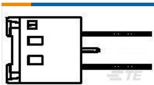
TE 产品编号3-178139-2 Header Assembly: Wire-to-Board, 15A, gold or tin plated
