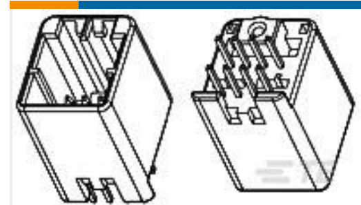
TE 产品编号1-1376137-2 Header Assembly: Wire-to-Board, 5A, gold plated
