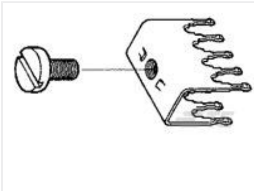
TE 产品编号580133-5 THREADED, PWR PIN, PLTD & LUBE
