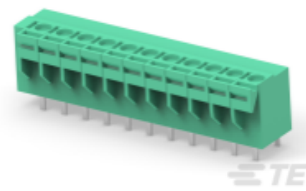
TE 产品编号 1-1776259-1 11P Spring TB, 180deg, VT,5mm, Green
