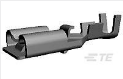
TE 产品编号179973-1 250 PL EX REC. 22-18AWG PTBR
