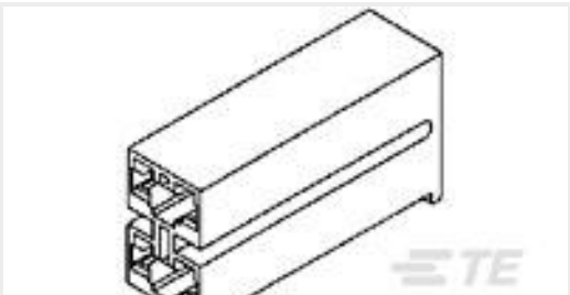
TE 产品编号175578-1 PL 187 HOUSING RECEPTACLE
