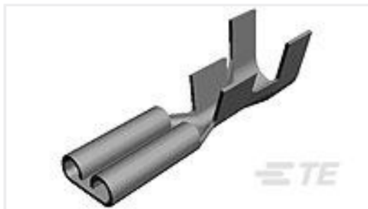
TE 产品编号 170043-2 110 FASTON, REC., 24-20 AWG, TPBR
