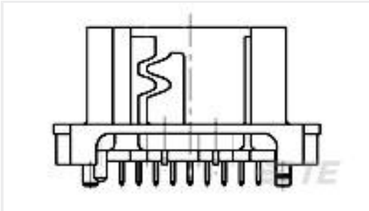
TE 产品编号967618-1 18pos MQS .63 header 180deg
