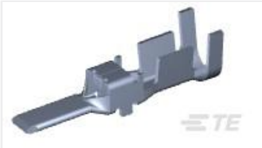
TE 产品编号1746974-1 GRACE INERTIA CONNECTOR 6.2 MM PITCH TAB
