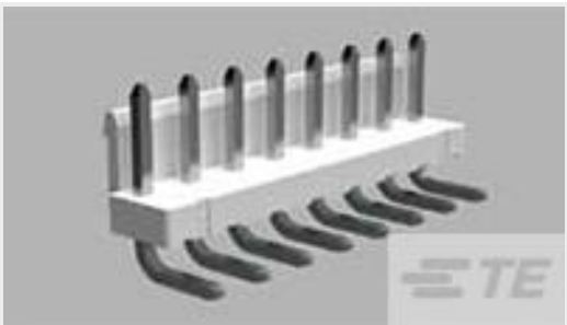
TE 产品编号1-1744428-2 3.96 EP HDR ASSY 12P R/A, GW
