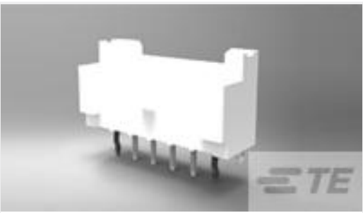
TE 产品编号1-2132415-5 EP2.5 Shrouded HDR ASSY 15P VERT w/oboss
