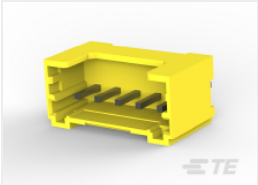
TE 产品编号3-1971032-5 5POS HEADER ASSEMBLY FOR GIC 2.0 EV
