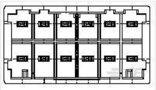
TE 产品编号2-1871571-3 GIC 3.3 HEADER ASSY 12POS
