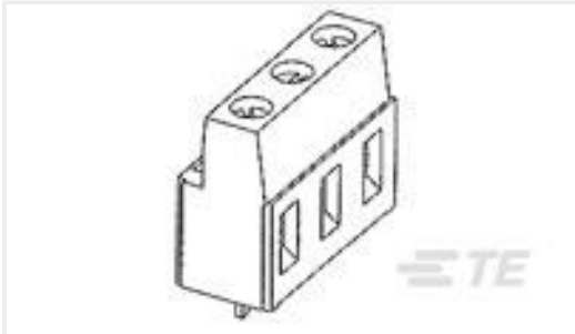
TE 产品编号282844-4 TERMI-BLOK PCB MOUNT 90 4P.
