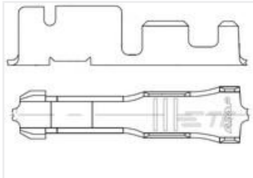
TE 产品编号2178453-1 .090 CLUSTER REC.
