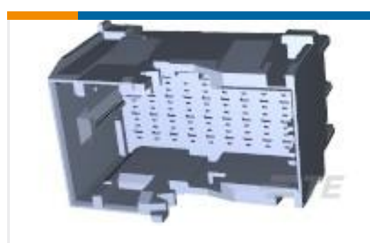
TE 产品编号1-1718492-3 1.5MM TAB HSG 36 POS ASSY
