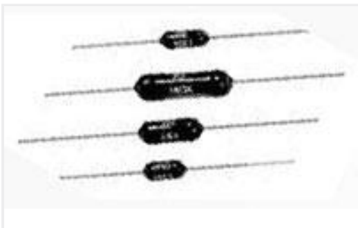
TE 产品编号2-1879663-9 H8 210R 0.1% 15PPM
