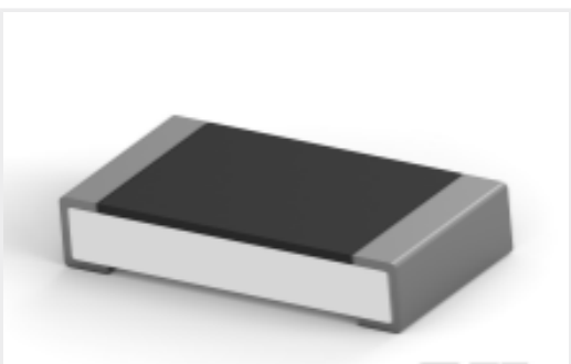
TE 产品编号2176388-5 RQ 1206 11R 0.1% 10PPM 5K RL
