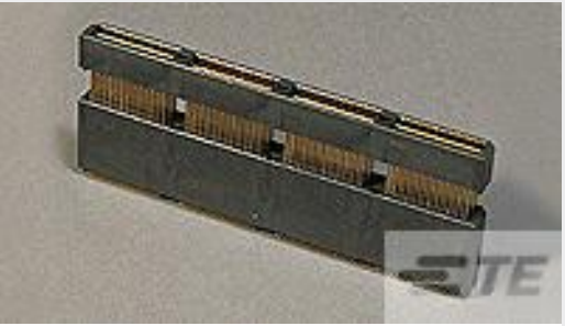
TE 产品编号 1-1658051-4 MSB0.80PL30ASY112DP,-,F,VCTY
