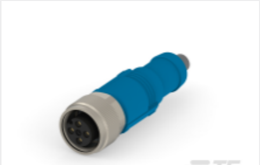
TE 产品编号T4151320004-005 RPC-M12-FS-4CON-PUR-5.0
