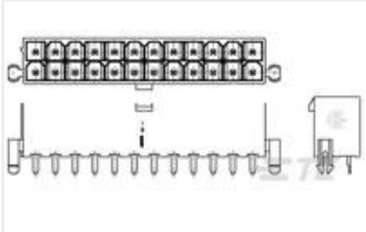
TE 产品编号1586040-4 4P VAL-U-LOK VRT HDR W/P V0
