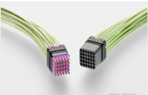
TE 产品编号ZPF0000000000202709 DMC-MR 30-23 SN
