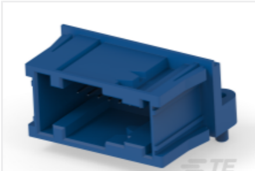
TE 产品编号6-1379731-3 18pos MQS .63 header 90deg THR
