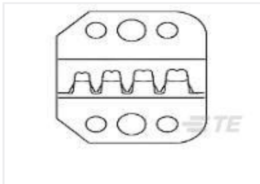
TE 产品编号91337-2 SIZE 16 PRO-CRIMPER DIE
