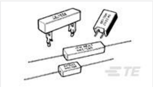
TE 产品编号2-1623779-3 SQB20 150R 5% (WIRE)
